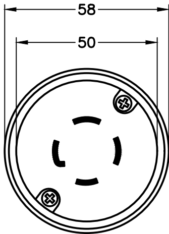
NEMA L15-30 PLUG FRONT VIEW
